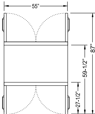
MPR524 PLAN VIEW
