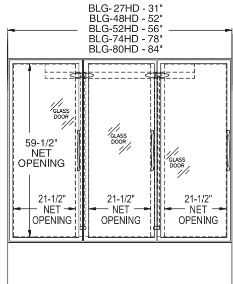
ELEVATION VIEW
